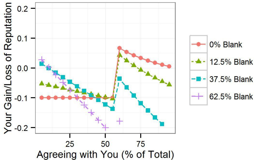
Figure 6. The “double-agent incentive”, where Voters prefer to falsely claim that they intend to attack. As long as >50% of the Voters are honest overall, each Voter wants (reward, vertical axis) to minimize the number of honest Voters (rival-Voters who agree with your true information, x axis). This discourages cartels and “voting pools”. The reward is indeed highest at 51% agreement; of course, this is perilous, as the 51% is just a few percentage points away from holding a bare minority view, which would net the lowest reward. This graphic also includes information about how this reward function reacts to a Voter’s failure to provide any data at all (see graph legend).
