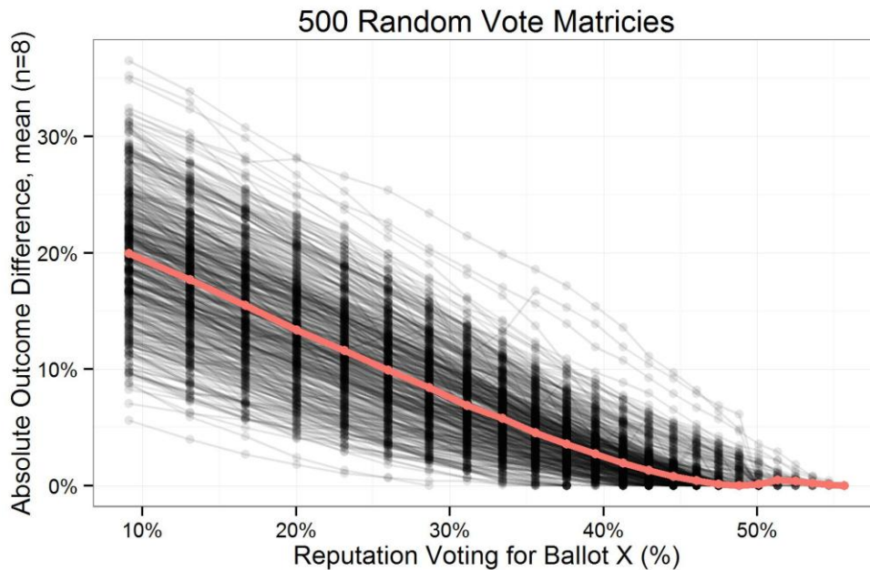
Figure 9. A graphical representation of 500 Vote Matrices, each 256 Ballots by 8 Decisions, consisting of entirely random data. The horizontal axis represents the disproportionate weight allocated to one Ballot, and the vertical axis represents how closely this Ballot matched with the final results. The red line indicates the average across all 500 trials, and clearly indicates that a large Votecoin majority is useless if the VTC-group is poorly coordinated. 22
