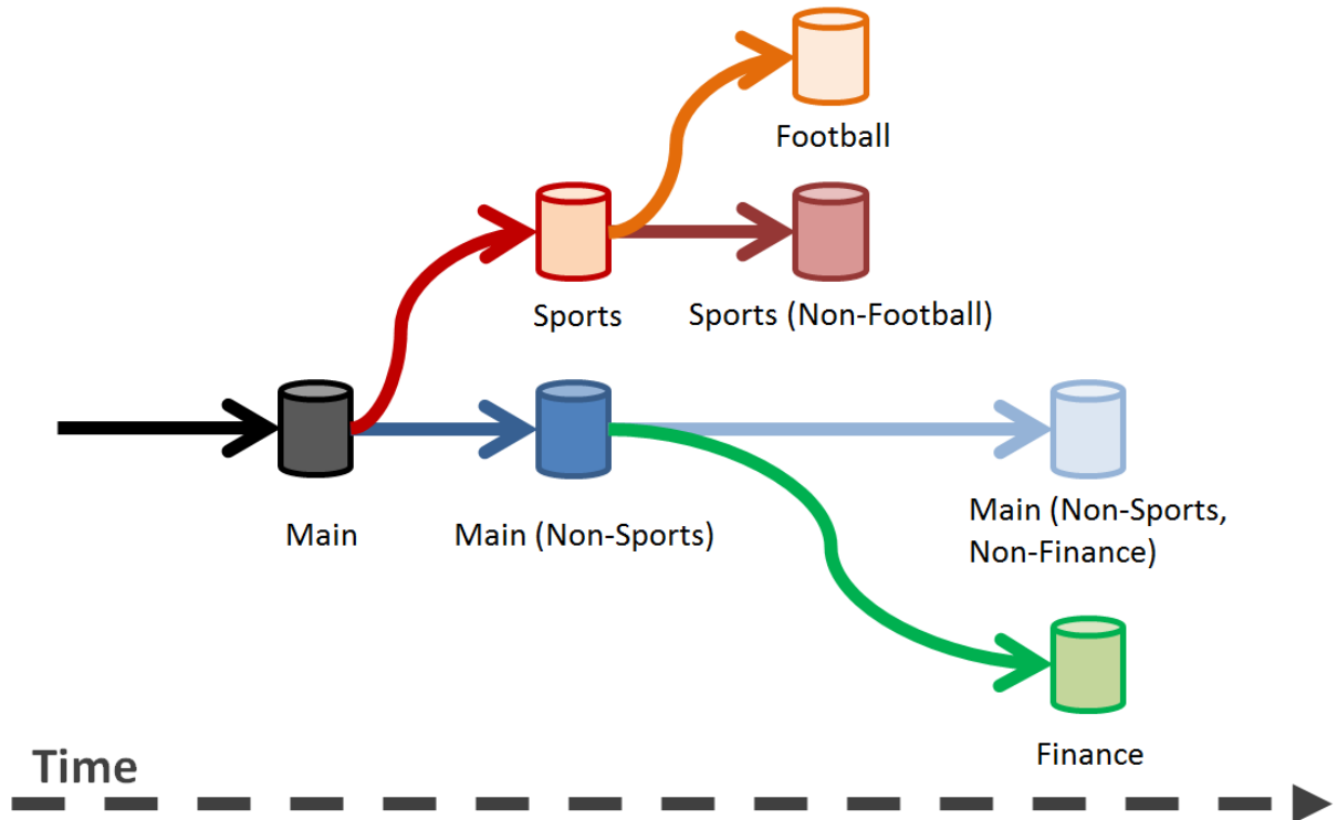
Figure 14. Holders of any Branch (cylinders) have a “free option” to own future branches. For example, anyone who owns 3 VTC on “Sport” will, when “Sport” splits, own 3 VTC on “Football” and 3 VTC on “Sports (Non-Football)”.
