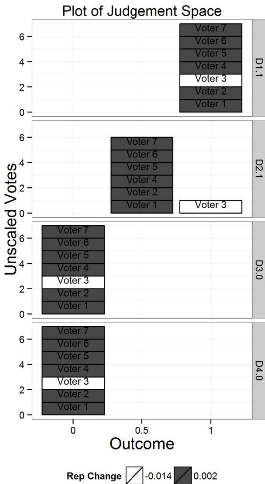
Figure 5. Two Vote Matrices and their corresponding SVD-Outcomes, represented graphically. Left, 7 Voters (matrix row, graph text-label), and right, 6 Voters. 4 Binary Decisions (matrix column, graph panel-row [right axis, above period, “D1”]), vote count (graph left axis), No/Yes outcomes (matrix cells, graph bottom-horizontal axes), consensus score (how well voters agreed with each other, graph darkness), and “correct” Outcome (graph panel-row [right axis, below period]).
