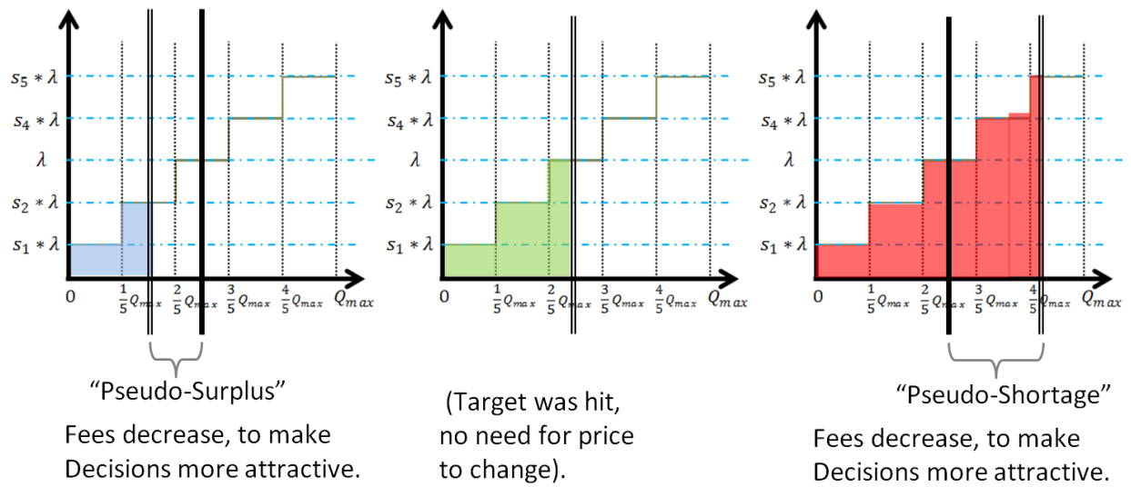
Figure 20. The effect of sales on Listing Fees. The central vertical black line intersects the horizontal axis at the target sale-quantity, and the double vertical black line represents the actual sales-quantity. When the target is hit exactly (center), \lambda_{t+1} does not change. When sales are under target (left), \lambda_{t+1} decreases, and when sales are above target (right), \lambda_{t+1} increases.
