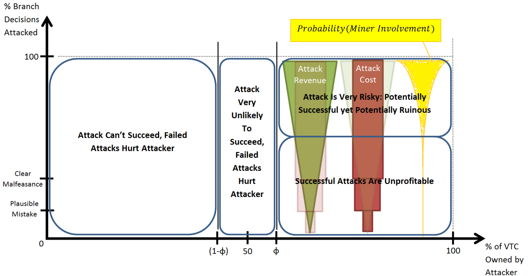
Figure 11. The more Decisions attacked, the easier it is to identify malfeasance (a few obvious mistakes gives away any “purposefully mistaken Ballot”). The Audit process sorts deviant Ballots into 5 maximally-representative clusters, meaning that attacking Ballots are very easy to identify. If Miners choose to involve themselves significantly, they will get the last word, meaning that there is some likelihood of the attacker failing disastrously: not only destroying the market capitalization of the VoteCoins of the attacked Branch (and increasing the value of VoteCoins of rival Branches), but also failing to mis-resolve any Decisions and thus granting the attacker zero revenue.
