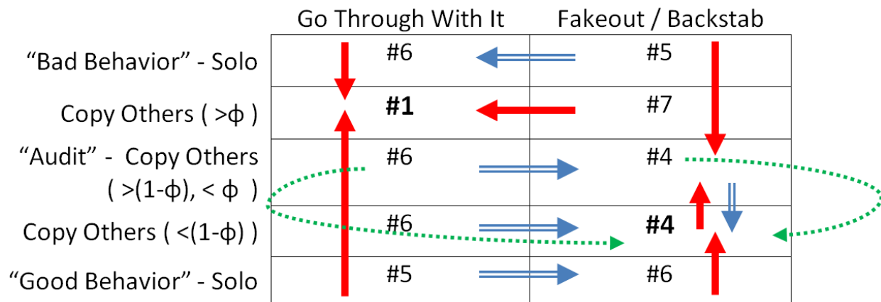
Figure 27. The same figure as before, but with the audit system added. A little friction halts the copy-inertia: The new cycle (green dashed loop) encourages individuals to lie about their claim to be copying (there is only one arrow: a Blue-Double). This de-emphasizes copying (blue arrows become stronger, red weaker), pushing the strategies toward the "Solo" rows, in this case holding them against the bolded cells. In particular, if we start with the information-less estimate of 50% copiers, the strategic logic carries us to the ("good") equilibrium.
