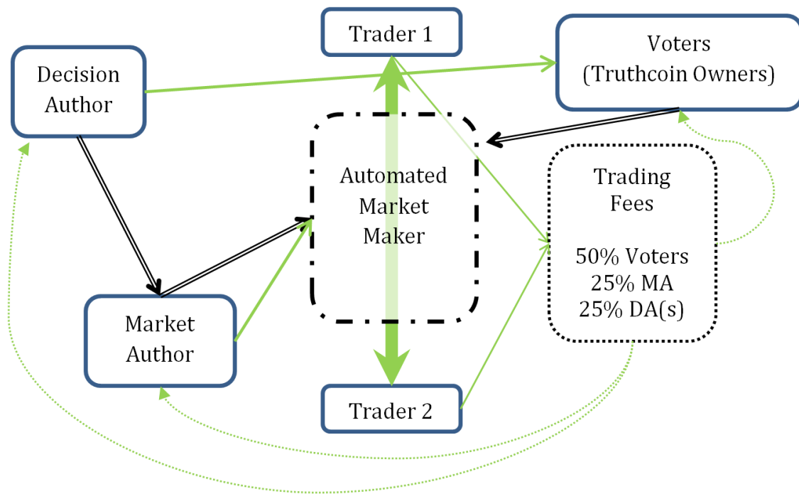
Figure 13. The flow of costs (green solid), revenues (green dashed), and information (black double) among various agents (blue solid) and accounts (black dashed). The horizontal axis corresponds to time, and line widths correspond to expected magnitudes, with the exception of revenues (whose magnitudes are a function of trading volume).
