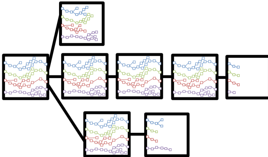
Figure 15. Blocks (large black squares) containing trades (small colored squares). Notice one orphaned block above the main blockchain and two below, but more importantly notice that each block contains many trade sequences for many Markets (colors). Some within-block sequences are themselves orphaned, but the trade-orphans are likely to be especially harmless (see below).
